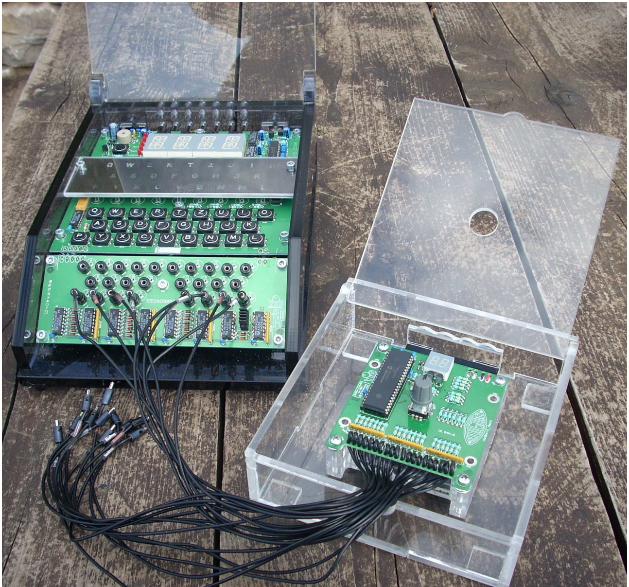
Enigma – E and Uhr attachment together. Enigma – E ed accessorio Uhr insieme.
